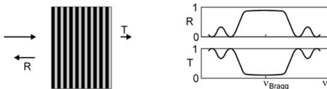
Fig. 25.3 Bragg reflector
