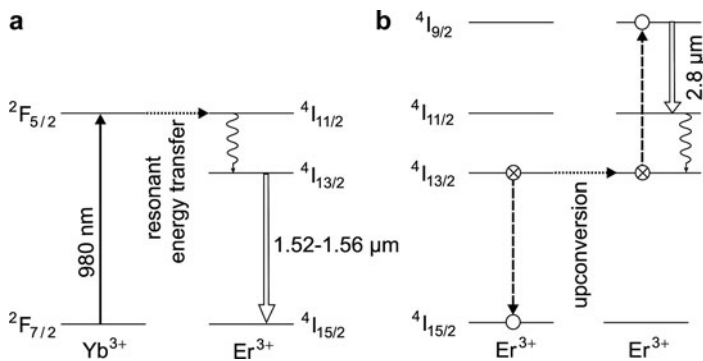
Fig. 15.10 Fiber lasers. (a) 1.5-μm erbium-doped fiber laser. (b) 2.8-μm erbium-doped fiber laser
