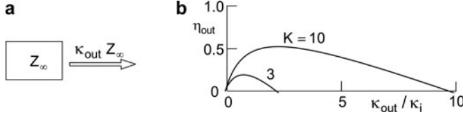
Fig. 8.5 Output coupling of radiation. (a) Output coupling coefficient. (b) Output coupling efficiency for two different pump rates
