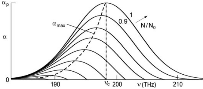
Fig. 18.15 Gain coefficient at different filling factors
