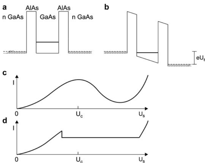
Fig. 31.11 Resonant-tunneling diode. (a) Quantum well. (b) Voltage-biased quantum well. (c) Hypothetical I - V curve. (d) I - V curve in the case of occurrence of feedback from a high frequency field
