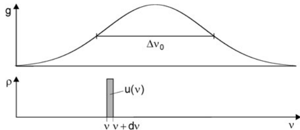
Fig. 7.1 Monochromatic radiation
