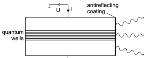
Fig. 34.1 Superluminescent LED
