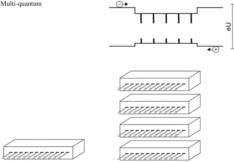
Fig. 22.11 Laser array and laser bar ( high-power semiconductor laser )
