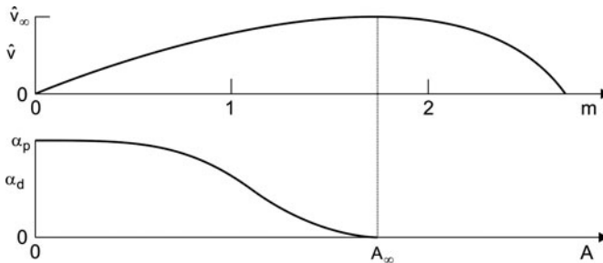
Fig. 32.9 Saturation behavior of a Bloch laser medium: dependence of the amplitude of the high frequency velocity ( upper part ) on the modulation degree, and dependence of the gain coefficient on the amplitude of the high frequency field ( lower part )
