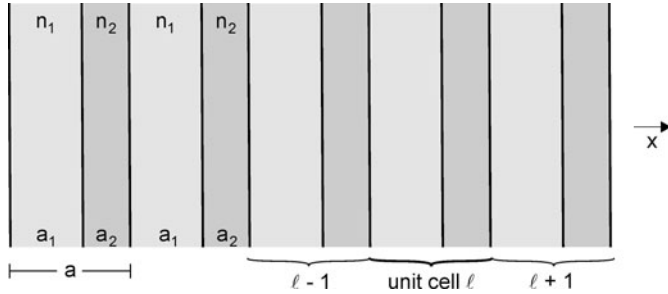
Fig. 25.10 One-dimensional photonic crystal
