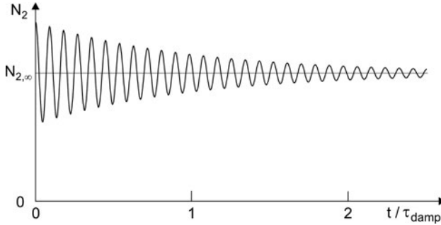
Fig. 8.8 Relaxation oscillation
