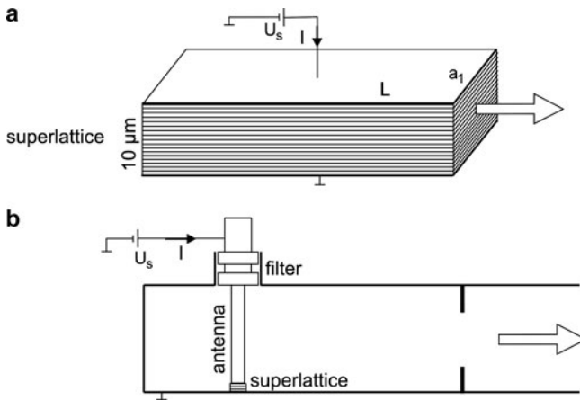
Fig. 32.15 Possible arrangements of a superlattice Bloch laser. (a) Large-area superlattice in a resonator. (b) Superlattice coupled to a resonator via an antenna
